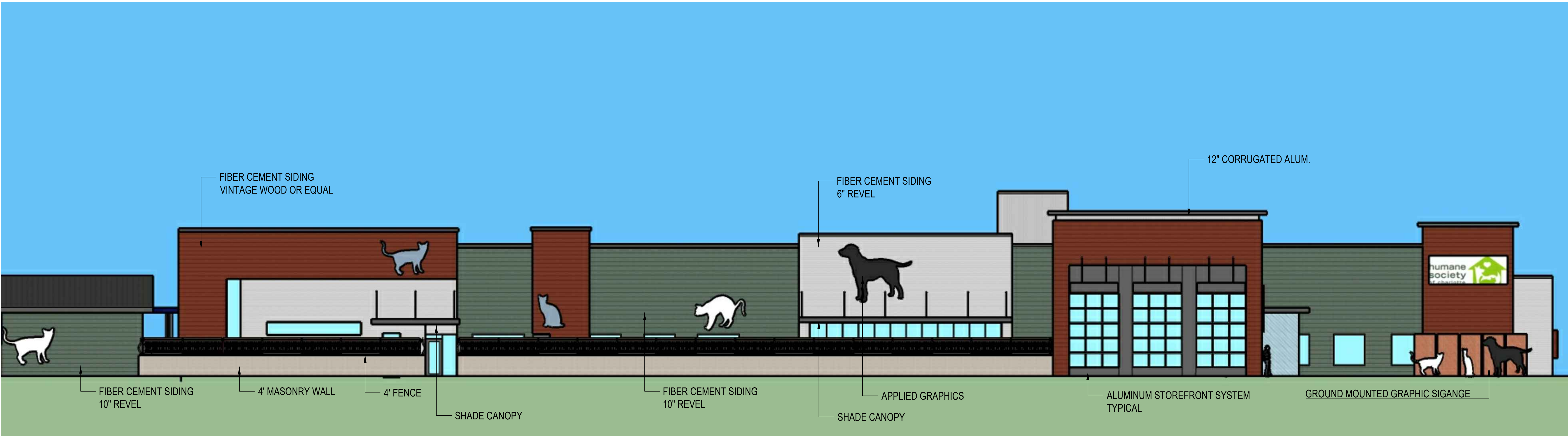
1 BERRYHILL ELEVATION 1/8" = 1'-0"
